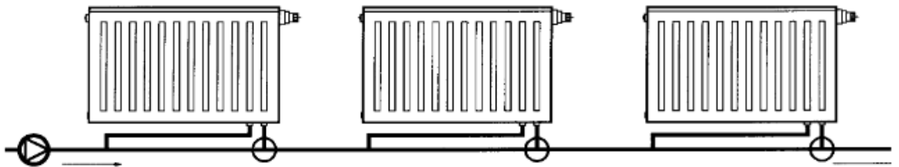
Option 3: One-Pipe System with Diverter Valves
