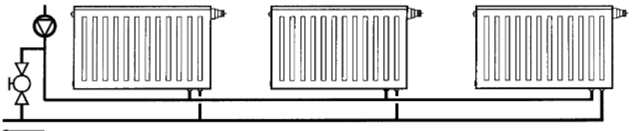
Option 5: Two-Pipe Reverse Return System
