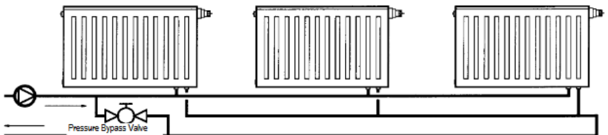
Option 5: Two-Pipe Reverse Return System
