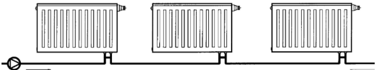
Option 4: Two-Pipe Direct Return System
