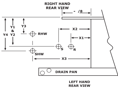
RIGHT HAND REAR VIEW
